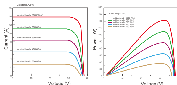
Current-Voltage & Power-Voltage Curves (RMHT54/405O2)
